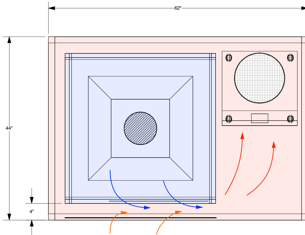
Top View: Airflow Pattern for HEPA In & HEPA Out Enclosure
